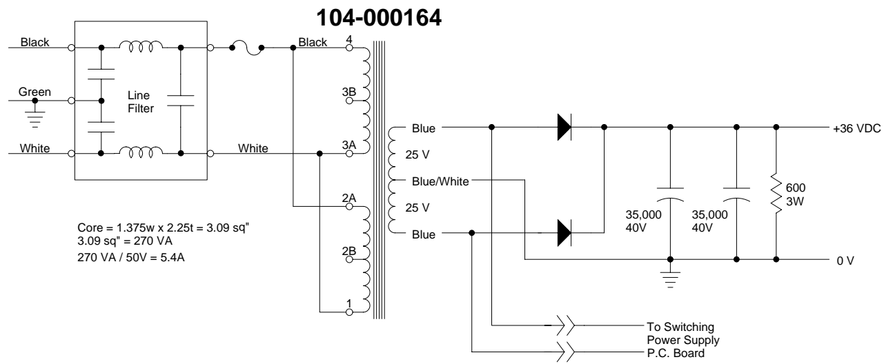
Transformer 104-000164 Assembly
