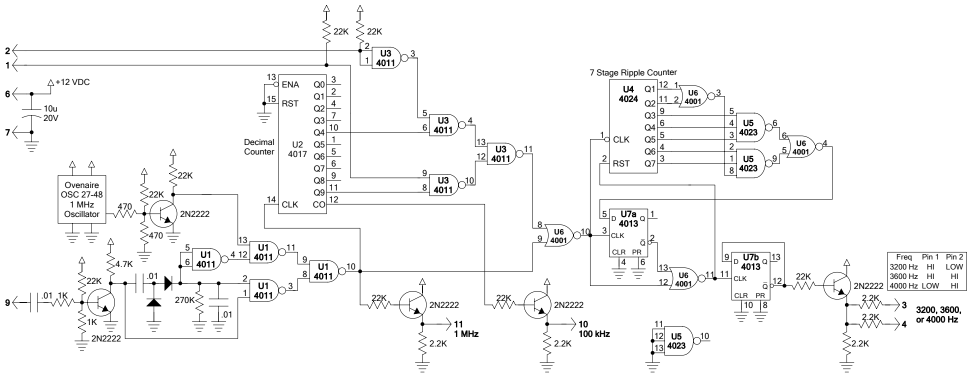
Ovenaire 1.000 MHz Oscillator Board Drawing by VE6SBS - www.sbszoo.com
